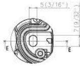
Detail D (2:1) Symmetrical
