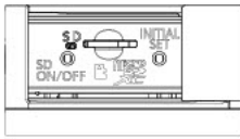
Inside of SD memory card cover (S=2:1)
