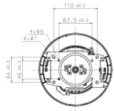
With Decorative cover & Camera mount bracket
