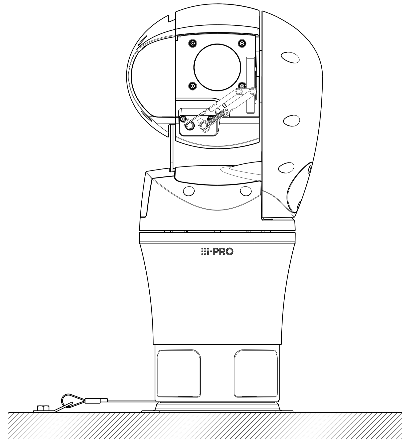
With attachment plate & safety wire (S=1:2)
