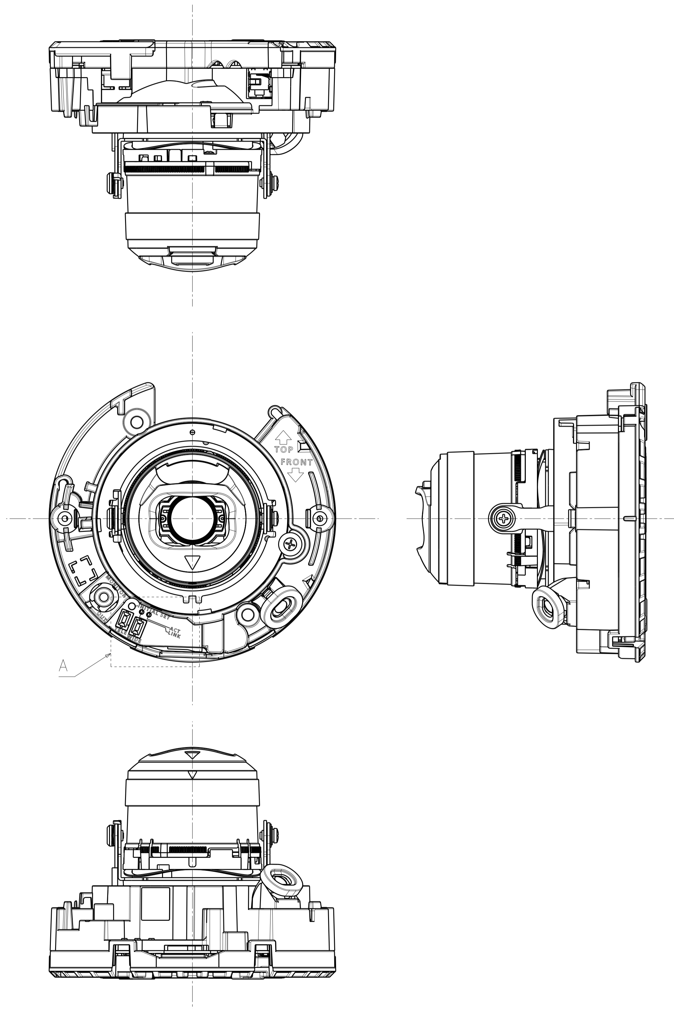
Without Enclosure
