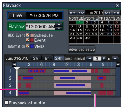
Playback slider
