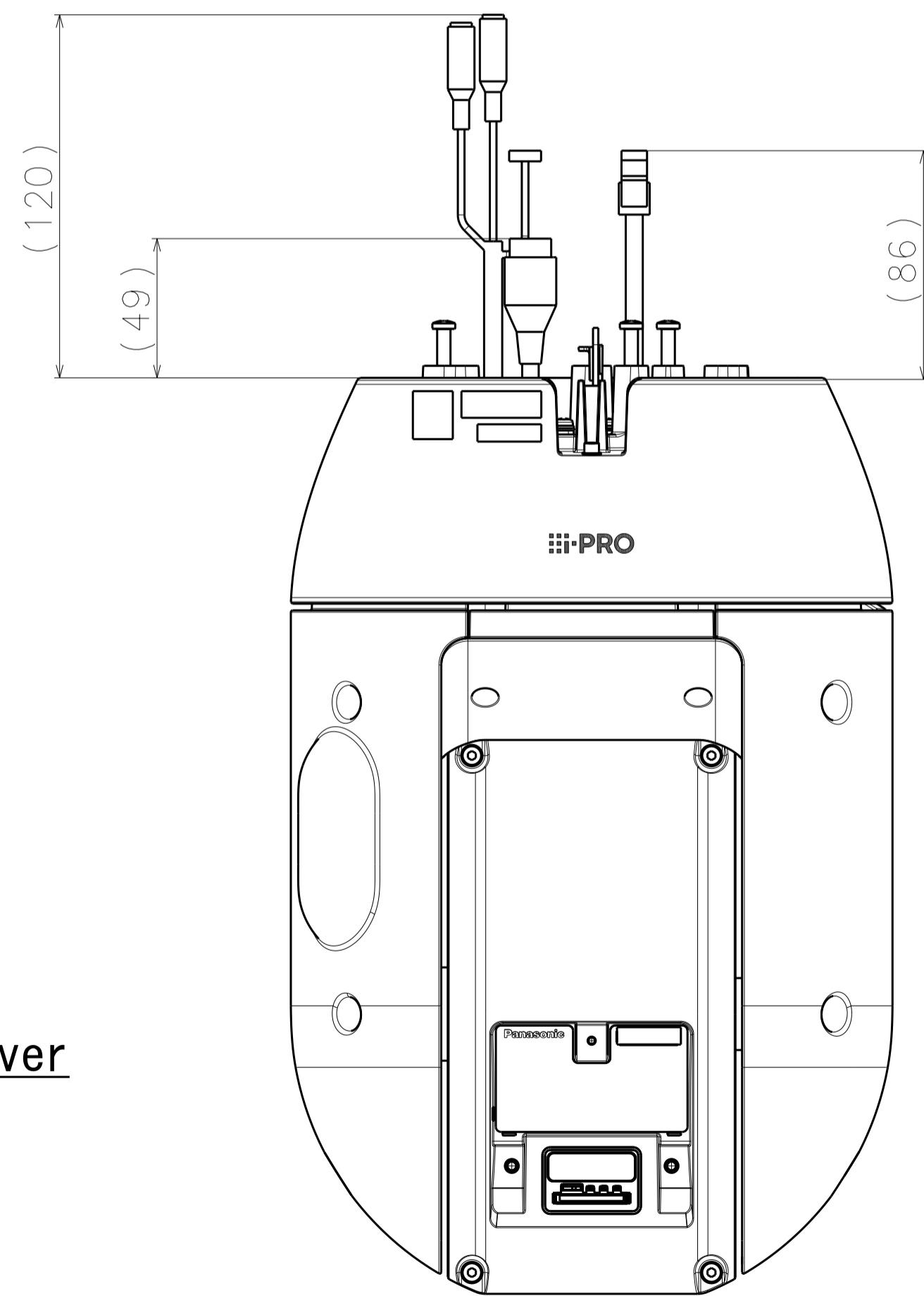
Remove SD slot cover / Cable cover
