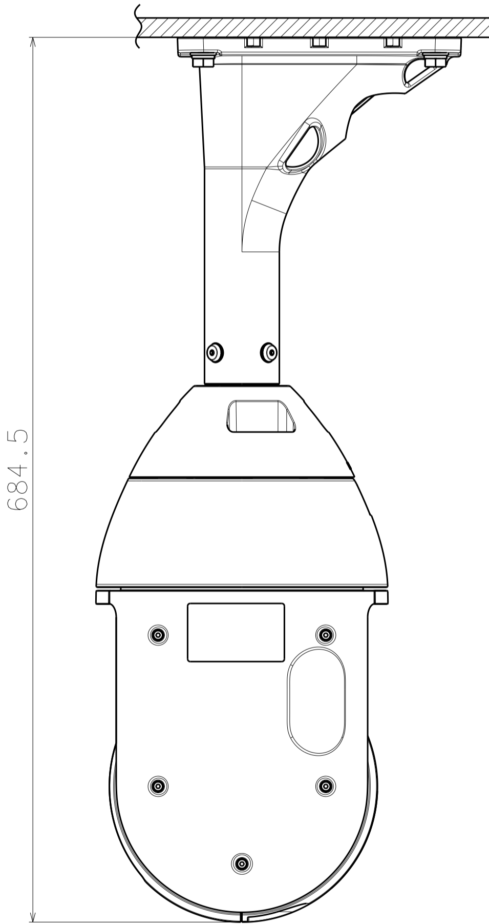
Attach to WV-Q121BS
