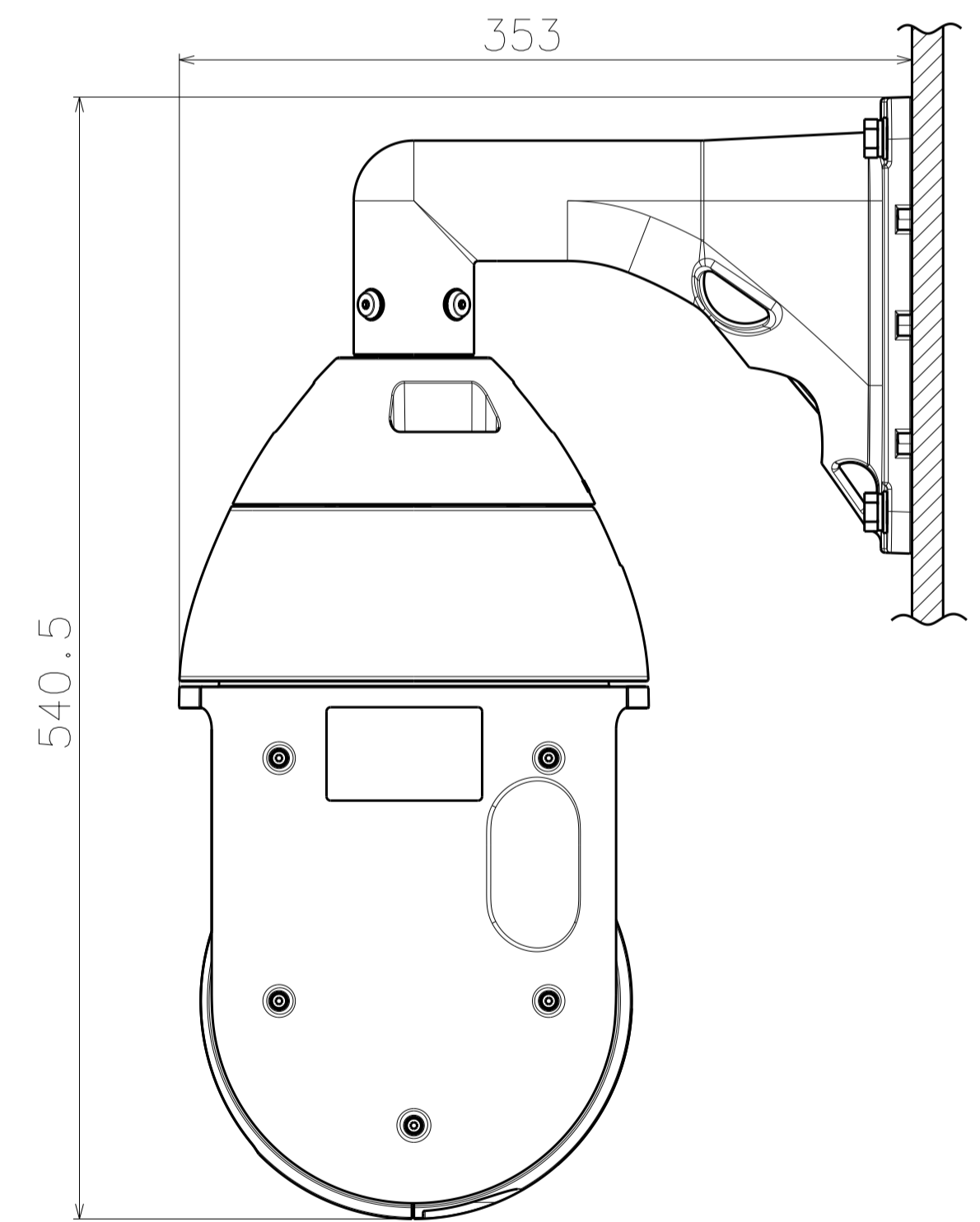
Attach to WV-Q122AS
