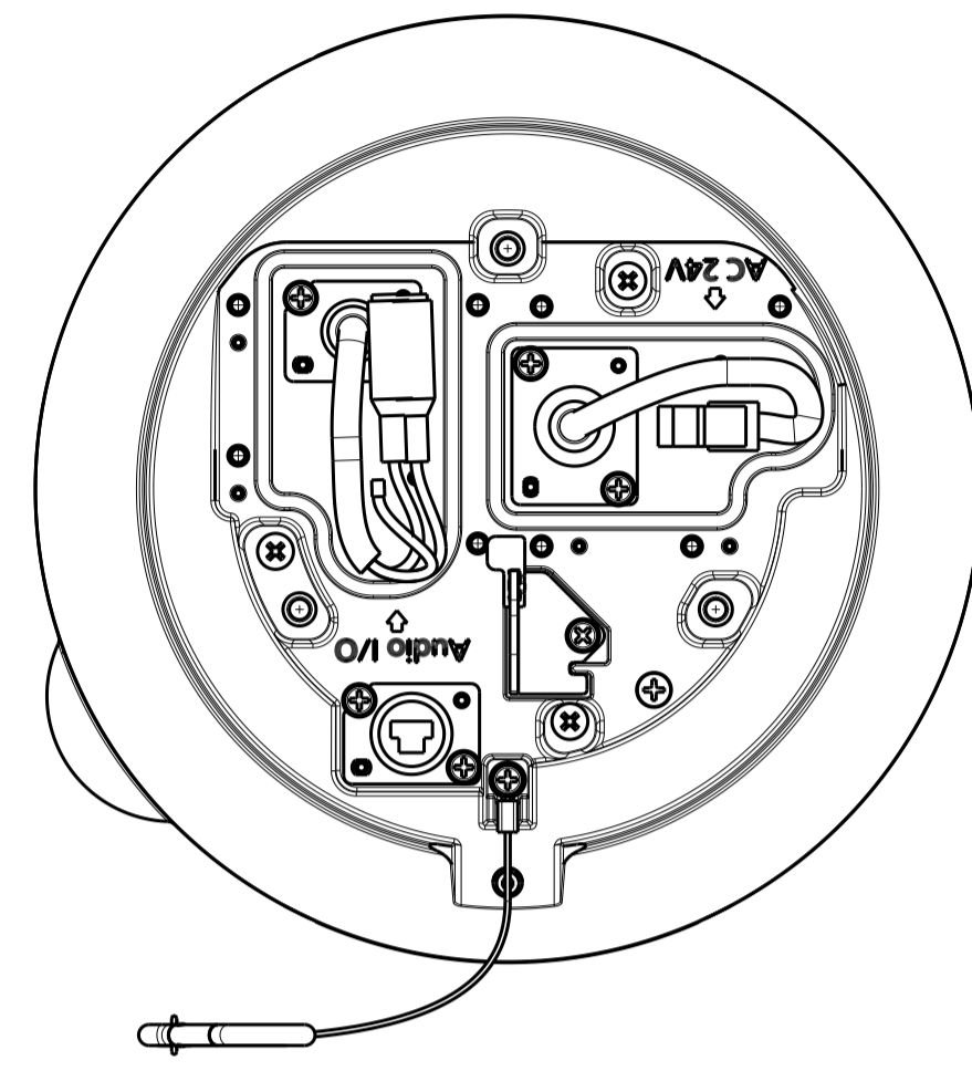
Remove Cable case
