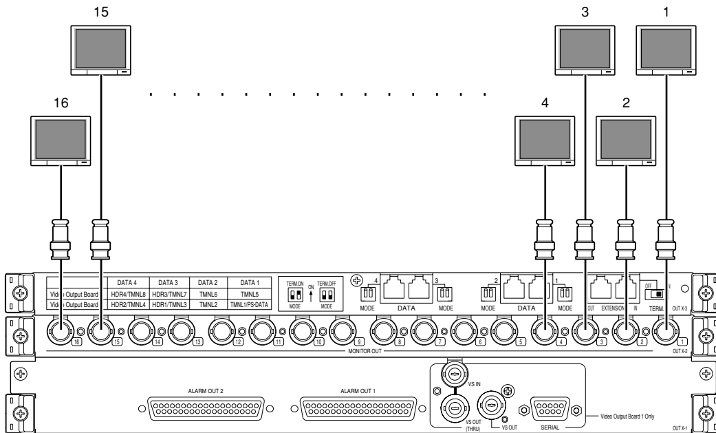
Hintere Video-Output-Boards
