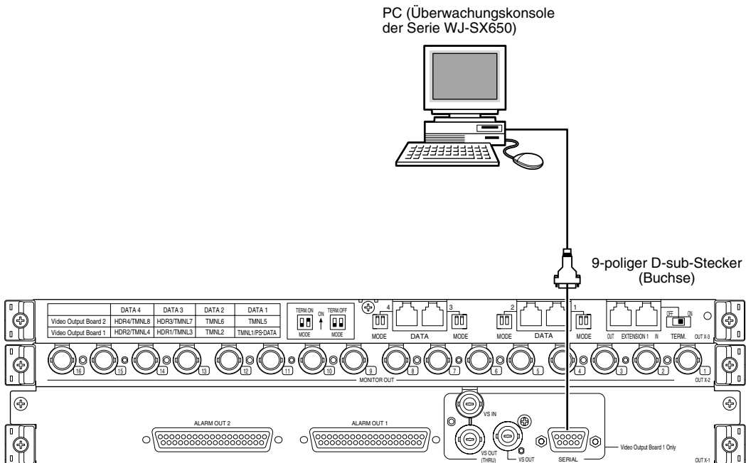
Hintere Video-Output-Boards
