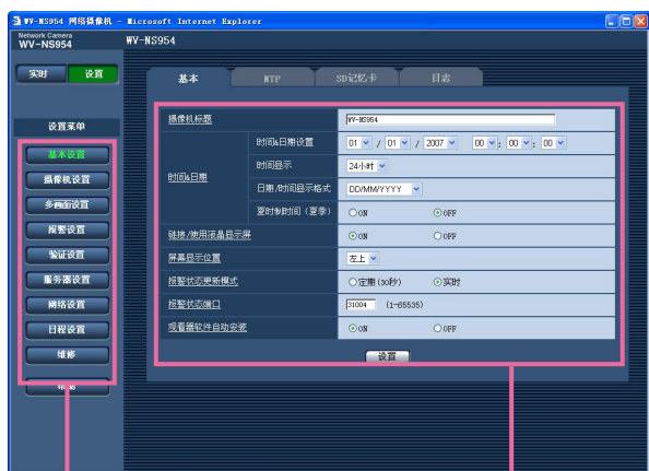
菜单按钮
