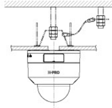
Attach to WV-QAT105A
