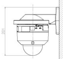
Attach to WV-QWL500-W
