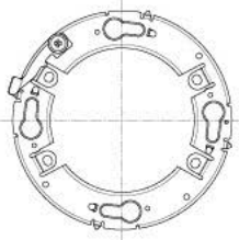
Attachment plate
